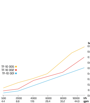
Pressure Loss
